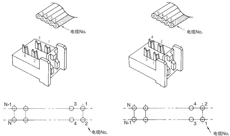
电缆No.配置 (TOP VIEW商品安装)
